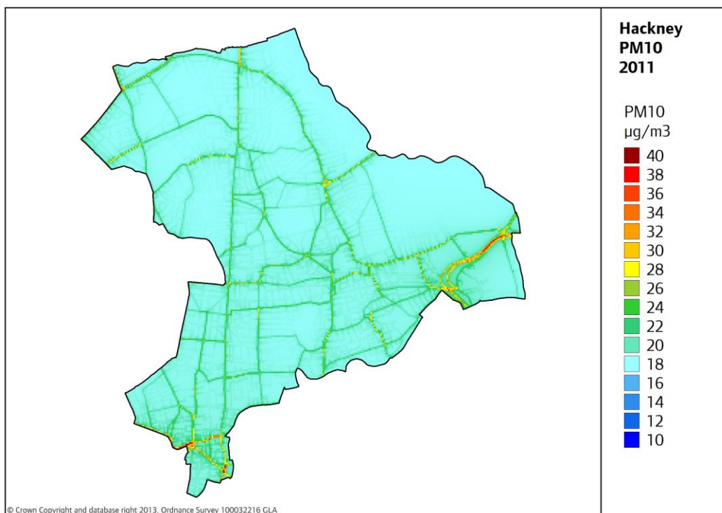
Image 5 Annual mean concentrations of PM 10 in LB Hackney 2011
