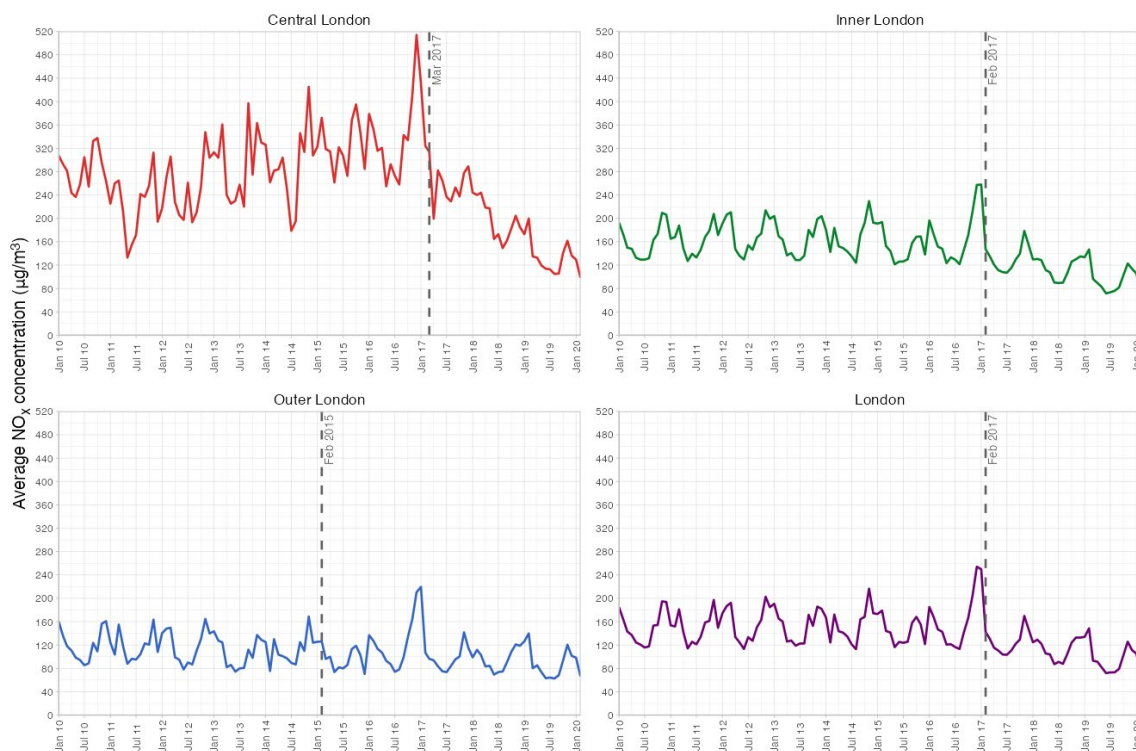
Figure 27: Average roadside NO x (Jan 2010 to Feb 2020) and detected change point by area
