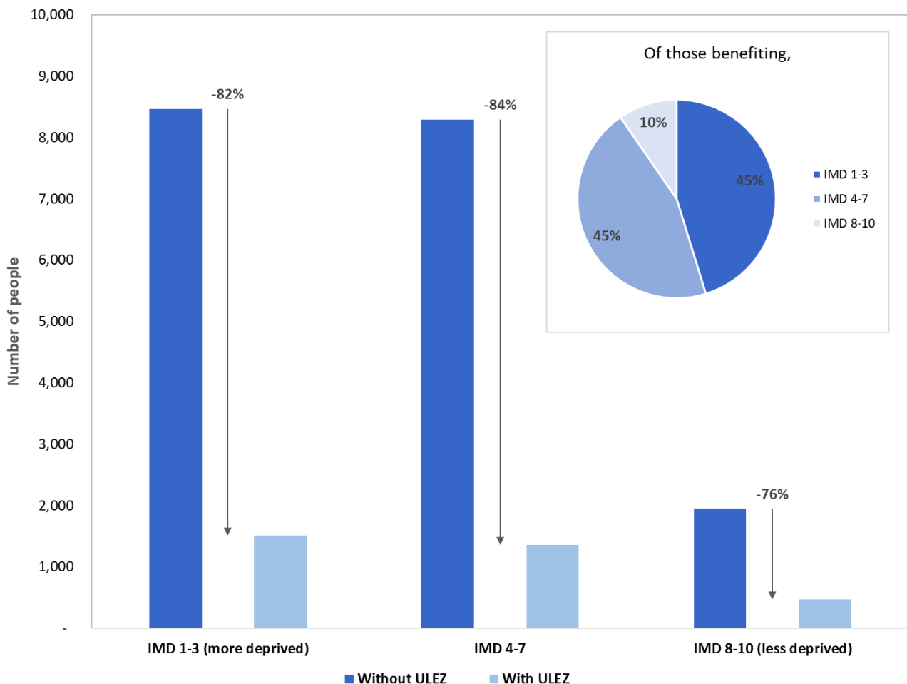
Figure 16: Change in population living by the TLRN in outer London, in areas where roadside NO 2 concentrations were predicted to exceed UK legal NO 2 limit (2023) with and without the impact of the ULEZ and its expansions, by IMD
