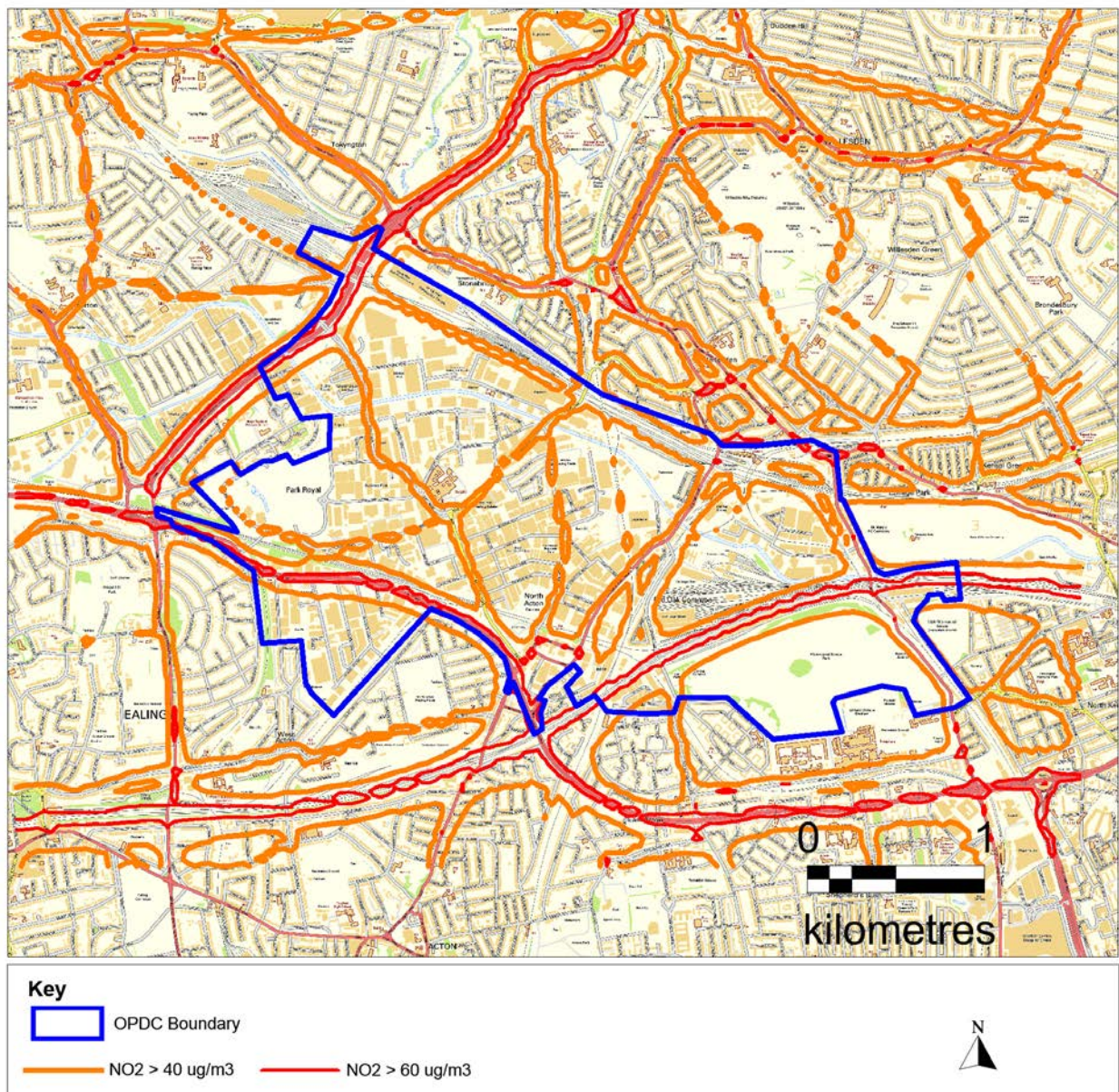
Figure 3.4 Contour map displaying LAEI NO 2 mapped concentrations
