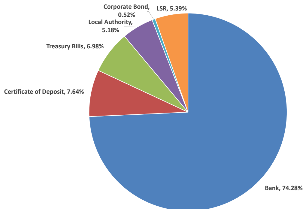
Instrument/Sector Breakdown
