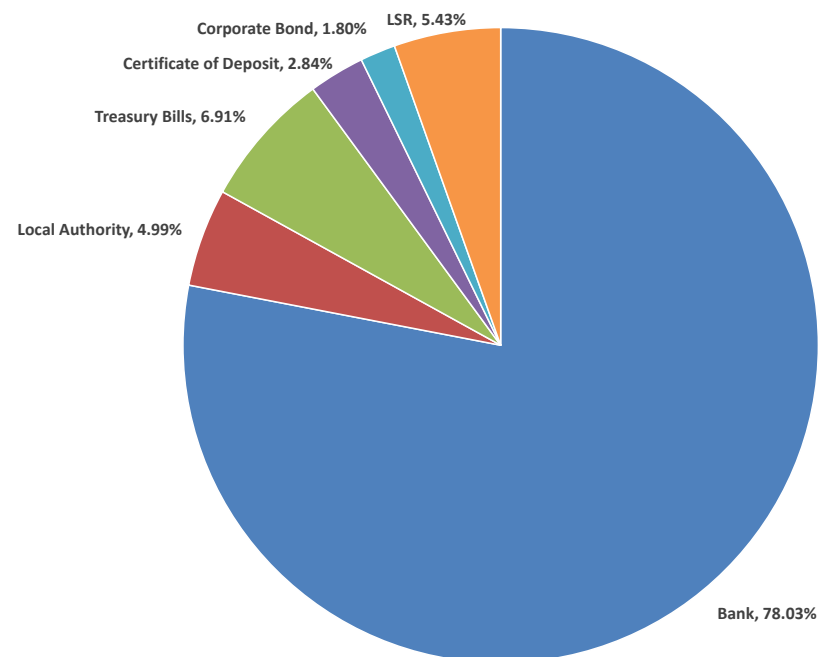
Instrument/Sector Breakdown
