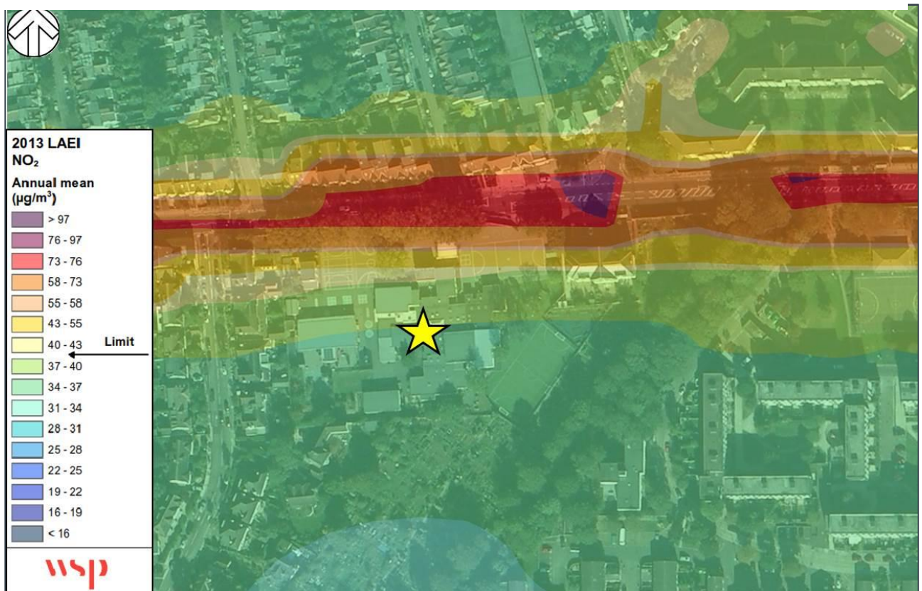
Figure 5 – Localised Air Quality modelling around East Sheen Primary School
